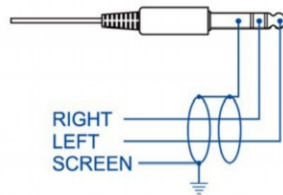
3.5mm HEADPHONE JACK
